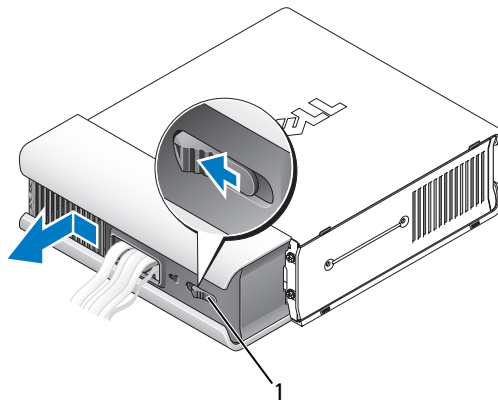
1 Frigöringsknapp
